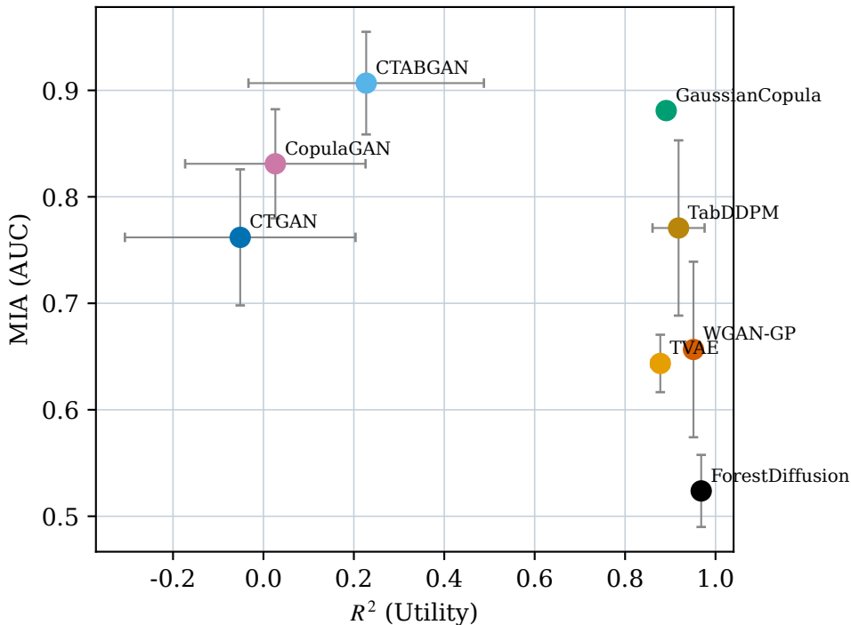
Energy Efficiency: R^2 (Utility) vs MIA (AUC)
